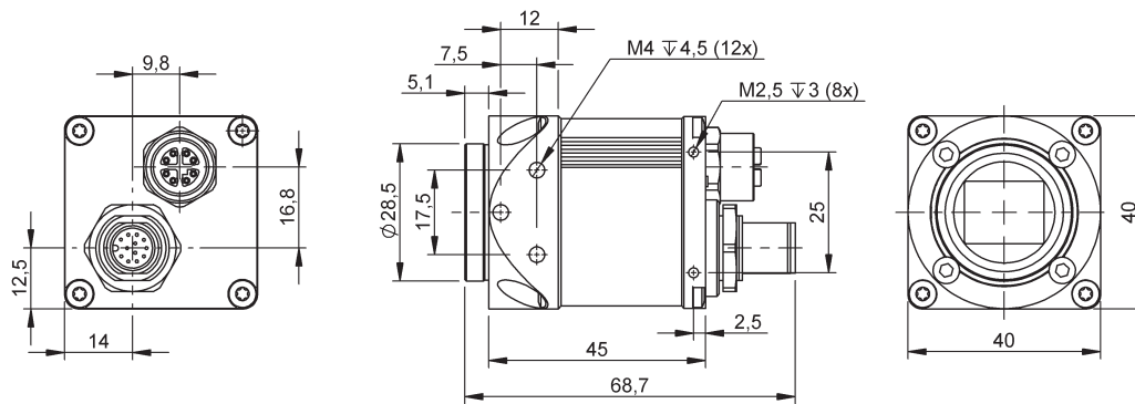
Dimensions in mm CS-mount is 5 mm shorter in length
